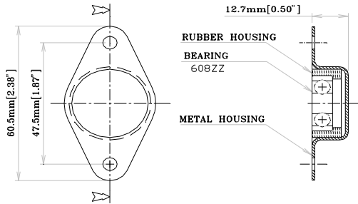
Housing for Ball Bearing
