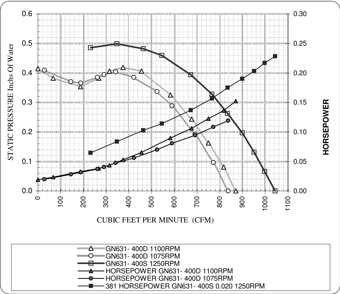
Blower Wheel Performance Curve
